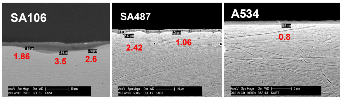
Fig. 3. (a) FAC rate and (b) SEM images of cross section for various materials after 3170 exposure
