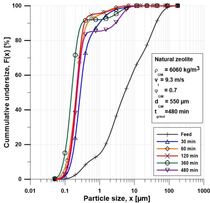
Fig. 1. Particle size distributions of the raw zeolite (feed) and ground products
