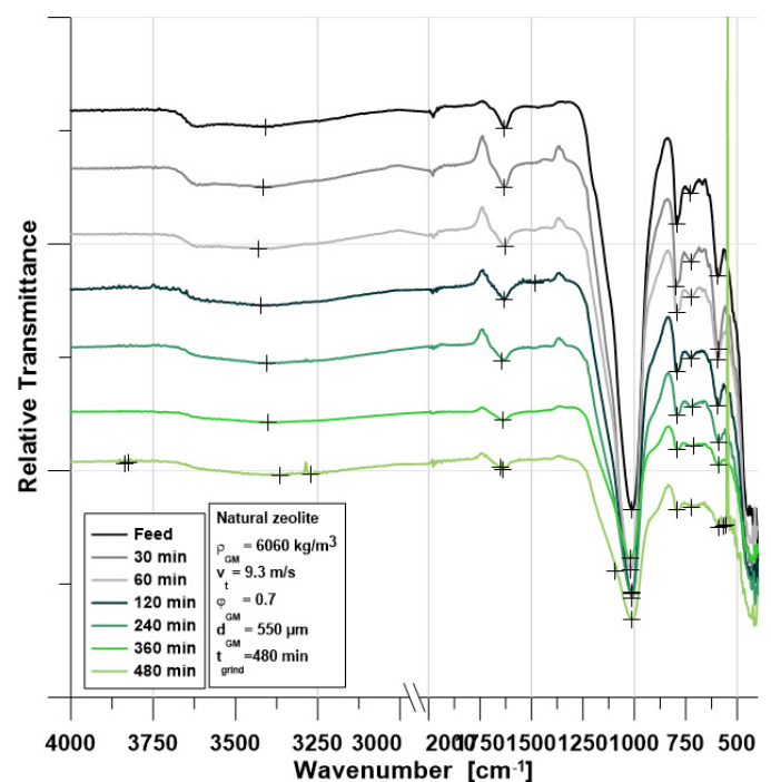
Fig. 7. FTIR spectra of zeolite samples during grinding
