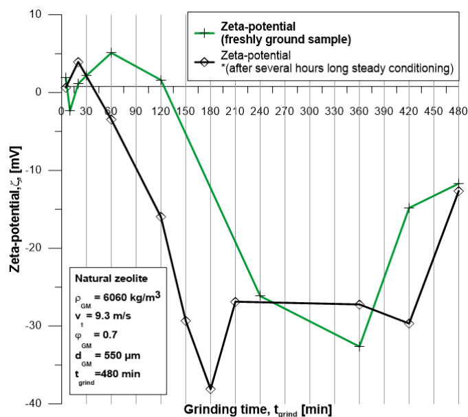
Fig. 10. Zeta-potential of zeolite during the continuous micro-grinding
