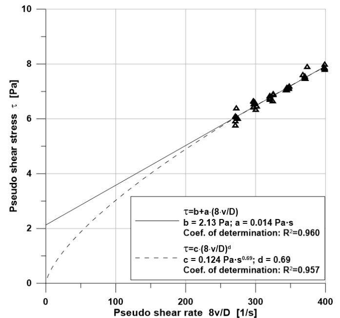
Fig. 6. The measured pseudo shear curve after 480 min long grinding
