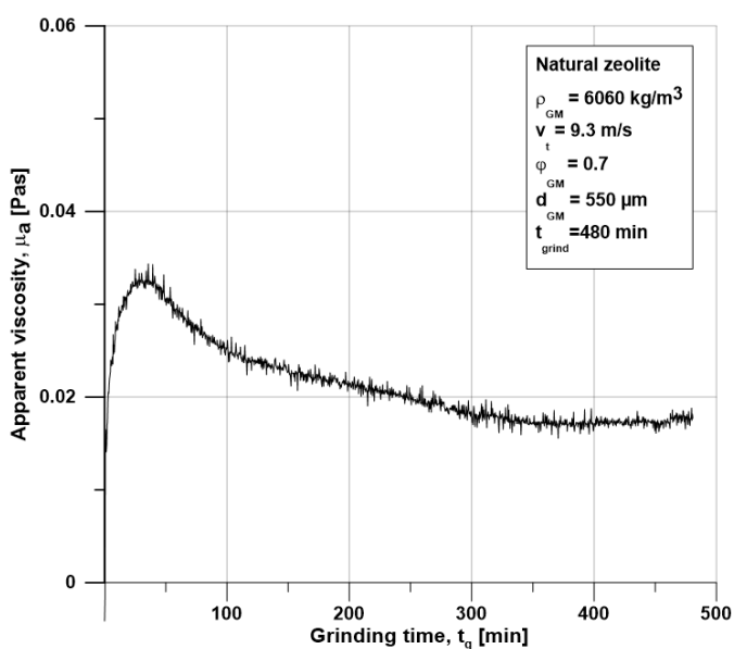
Fig. 5. Apparent viscosity of the ground suspension as function of time
