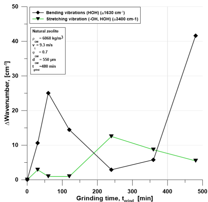
Fig. 8. FTIR peak shifting during grinding at 1630 and 3400 \text{cm}^{-1} wavenumber
