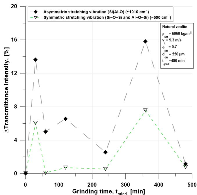
Fig. 9. FTIR peak intensity changing during grinding at 1010 and 590 \text{cm}^{-1} wavenumber
