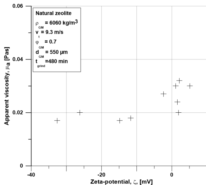
Fig. 11. Zeta potential as a function of apparent viscosity
