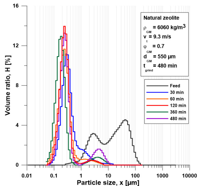
Fig. 3. Histograms of raw zeolite and ground products
