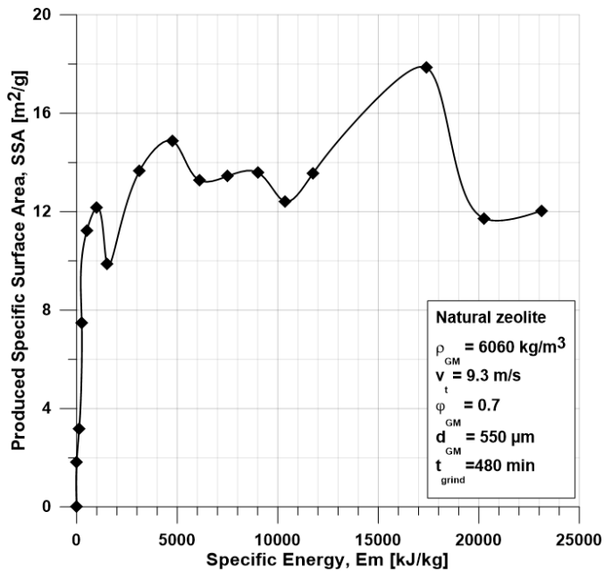
Fig. 4. The calculated specific surface area as a function of the specific energy
