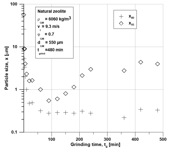
Fig. 2. The x_{80} and x_{95} particle size of zeolite during grinding
