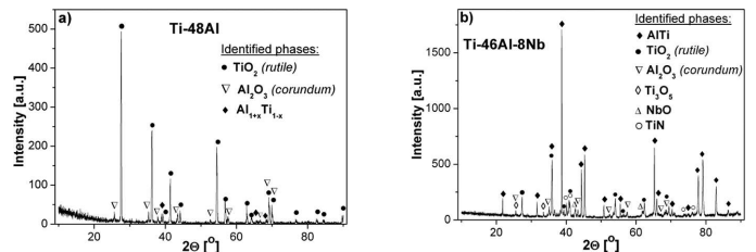
Fig. 2. X-ray Diffraction (XRD) analysis obtained on the surface of a) Ti-48Al and b) Ti-46Al-8Nb after isothermal oxidation at 1073 K in synthetic air
