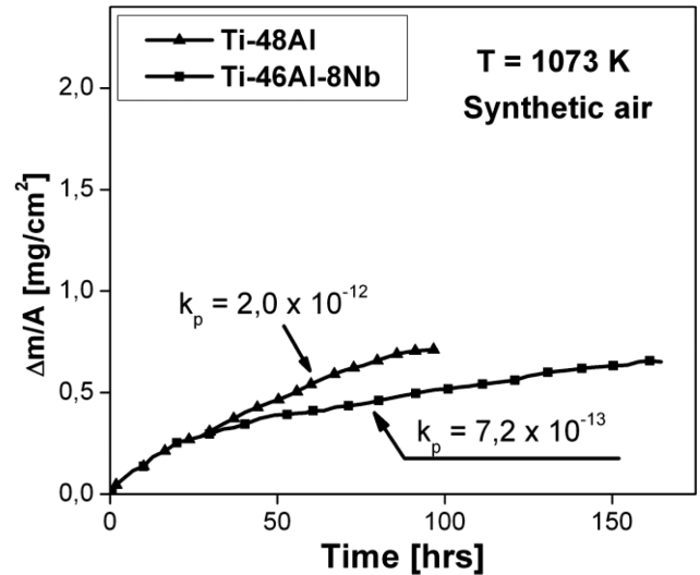
Fig. 1. Isothermal oxidation kinetics of Ti-48Al and Ti-46Al-8Nb at 1073 K in synthetic air ( k_p unit: \text{g}^2 \text{cm}^{-4} \text{s}^{-1} )
