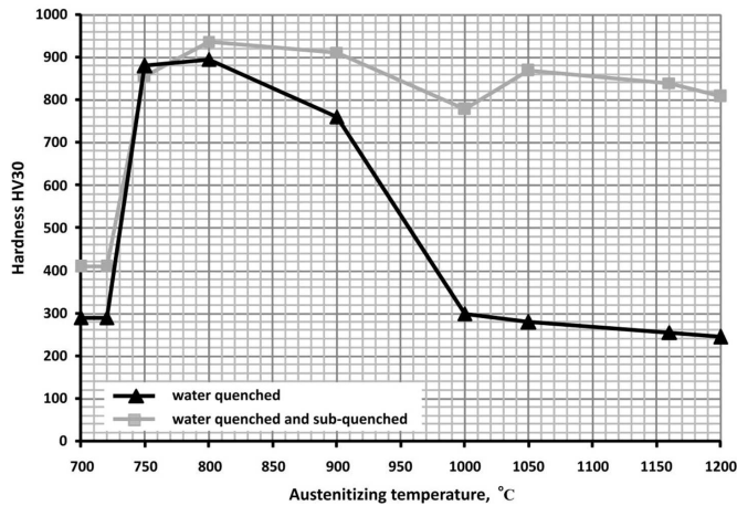
Fig. 1. Influence of the austenitising temperature on the hardness of the previously annealed and then quenched in water and of the quenched and sub-quenched in liquid nitrogen the new steel samples
