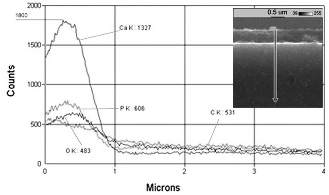
Fig. 5. Cross section and EDS line scan of the C/HAp coating deposited by sol-gel method on AISI 316L steel
