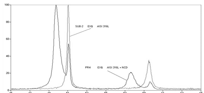
Fig. 1. Diffraction of 316L sample before and after deposition of the carbon layer
