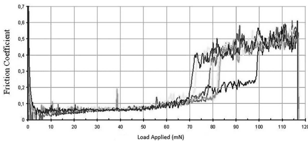
Fig. 3. Measurements of adhesion of carbon layer to AISI 316L steel base
