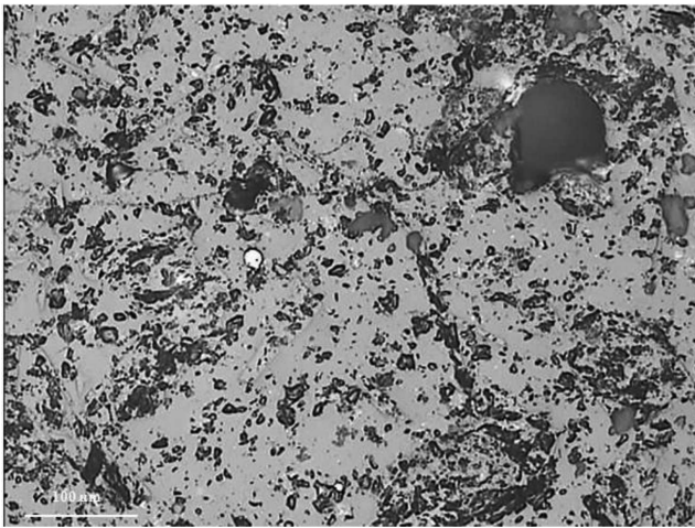
Fig. 5. Waste after the production of cast steel; metallic precipitations (with high reflexivity) and fine crystallites in glaze; reflected light, magnification 100x, one nicol
