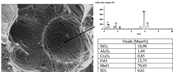
Fig. 8. Solid solution of FeO-MnO crystallized in pore of slag after the production of cast iron (SEM, EDS spectrum with chemical analysis)
