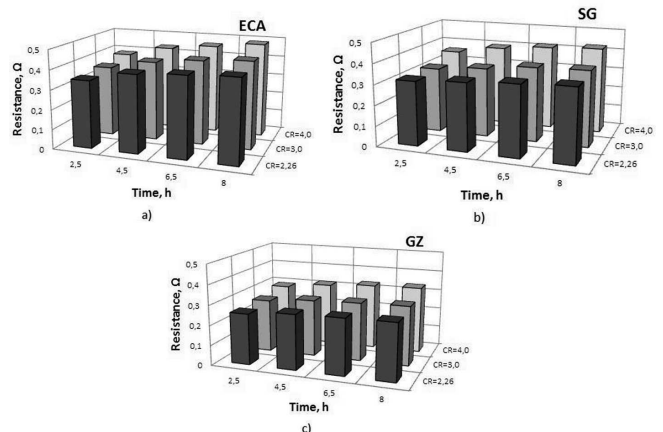
Fig. 7. Influence of the melt composition on the resistance changes in C/Al/electrolyte system for: a) ECA, b) SG and c) GZ
