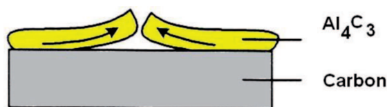
Fig. 10. Spalling carbide layer as a result of compression ( R_{P-B} > 2 )
