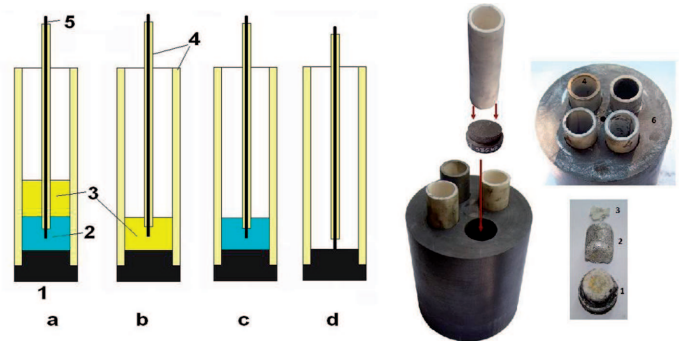
Fig. 5. Details of experimental cell for resistance measurements: 1- carbon lining sample, 2- aluminium, 3- electrolyte, 4- sintered alumina tube, 5- Mo wire, 6- graphite crucible, used in four systems: a)- carbon/Al/electrolyte; b)- carbon/electrolyte; c)- carbon/Al; and d)- “short circuit” of Mo electrode on cathodic carbon
