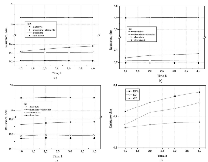
Fig. 6. Changes of electric resistance for: a) ECA; b) SG; c) GZ in four systems, and d) resistance comparison of tested samples in system with aluminium and electrolyte
