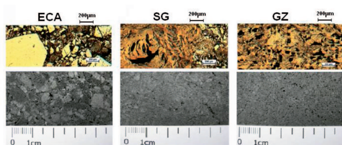
Fig. 2. Surface of the cathodic lining samples
