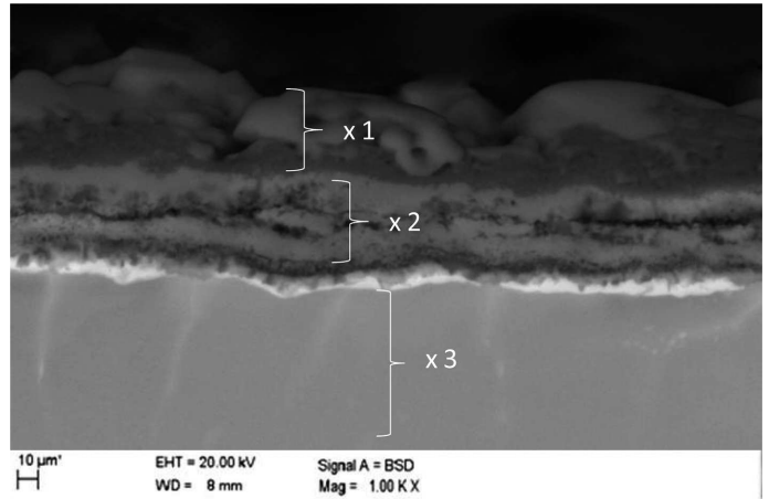
Fig. 16. Cross-section of the scale formed on Ti-46Al-7Nb-0,7Cr-0,1Si-0,2Ni coated with AlCrN after isothermal oxidation in air at 950°C
