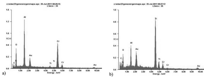
Fig. 14. EDX analysis results: (a) in area inside the rectangle #A according to Fig. 10 and (b) in area inside the rectangle #B according to Fig. 10
