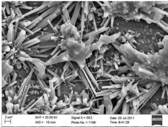
Fig. 13. The surface inside the rectangle #A according to Fig. 12
