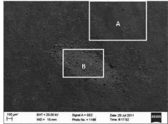
Fig. 10. The surface Ti-46Al-7Nb-0,7Cr-0,1Si-0,2Ni with AlCrN layer applied after isothermal oxidation in air at 950°C
