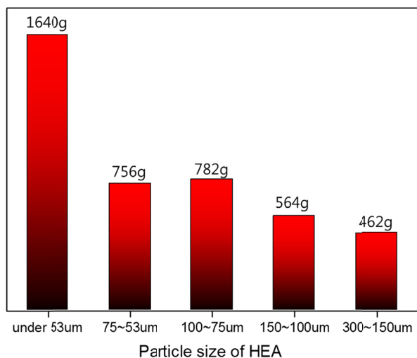
Fig. 1. Powder size distribution of gas atomized CoCrFeNiMn HEA powder
