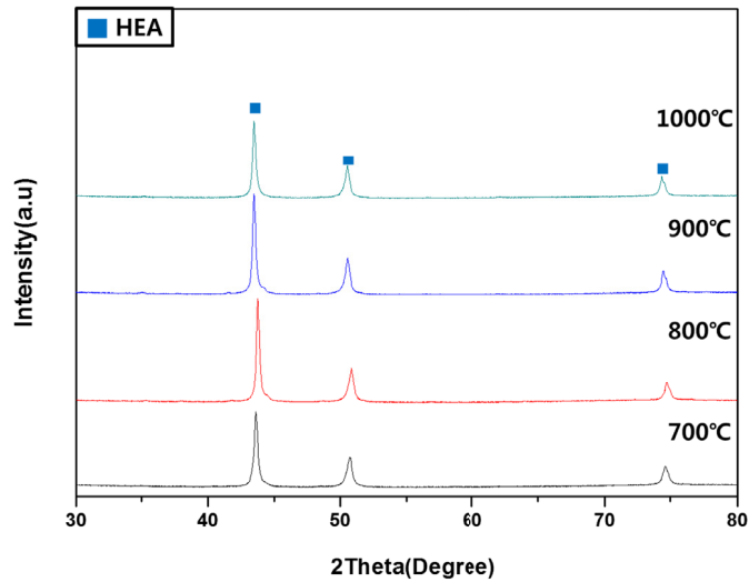
Fig. 5. XRD analysis of the SPS sintered CoCrFeNiMn HEA
