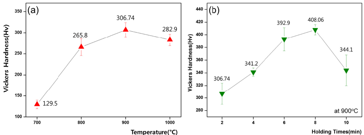
Fig. 6. Vickers hardness change of SPS sintered body (a) by the sintering temperature and (b) by the sintering time at 900°C
