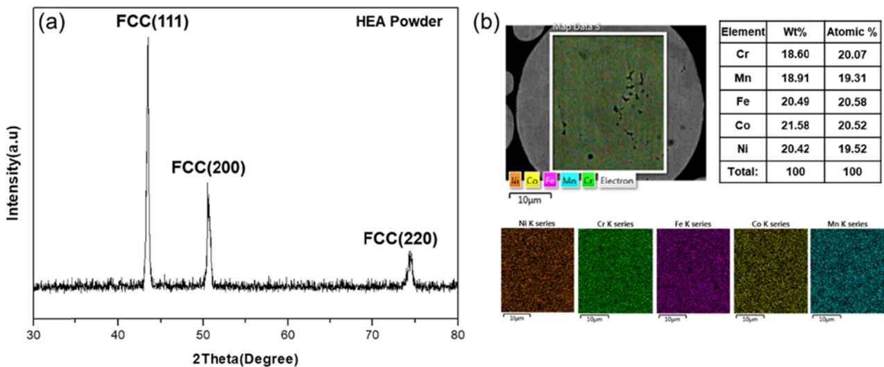
Fig. 3. Structural and elemental analysis of atomized HEA powder (a) XRD analysis of the powder, (b) polished inner surface of the powder
