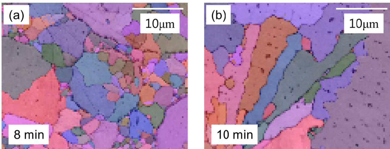
Fig. 7. EBSD images of sintered body, (a) 8 min, and (b) 10 min of sintering time
