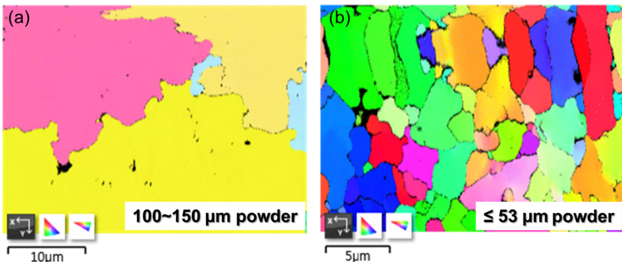
Fig. 4. Cross-sectional EBSD images of the atomized powders (a) 100~150 \mu\text{m} large sized powder, (b) <53 \mu\text{m} small sized powder
