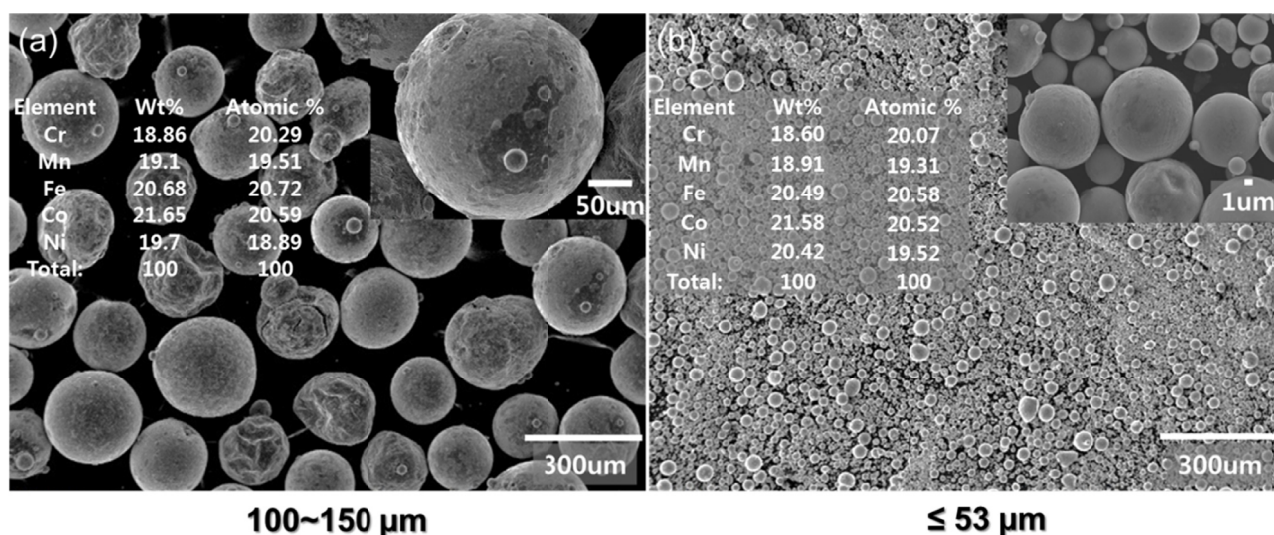
Fig. 2. Microstructure and surface elemental analysis of atomized HEA powder (a) 100~150 \mu\text{m} large sized powders, (b) <53 \mu\text{m} small sized powder
