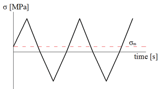
Fig. 1. The stress-time relation for the ratchetting phenomenon
