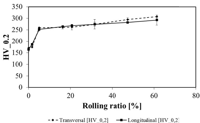
Fig. 6. Influence of rolling ratio on microhardness of ESFed CuSn bronze
