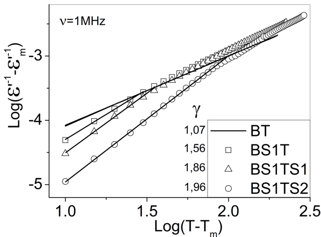
Fig. 9. The dependence of \log(1/\epsilon' - 1/\epsilon'_m) on \log(T - T_m) for BT, BS1T, BS1TS1 and BS1TS2 samples at chosen frequency 1 MHz
