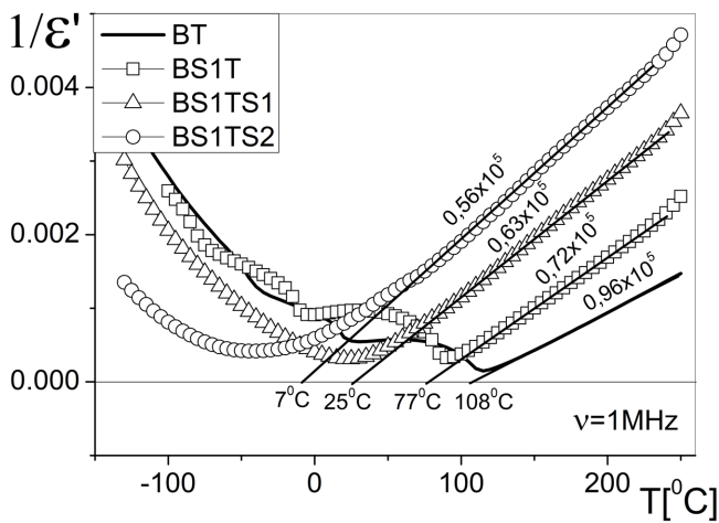
Fig. 8. The inverse of the real part of dielectric permittivity ( 1/\epsilon' ) as a function of temperature for BT, BS1T, BS1TS1 and BS1TS2 samples at chosen frequency 1 MHz
