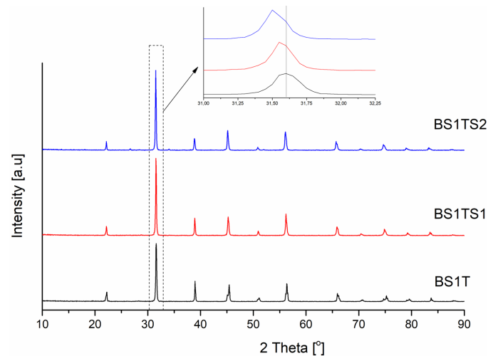
Fig. 4. Comparison of X-ray powder diffraction patterns of BS1T, BS1TS1 and BS1TS2 solid solutions powders prepared by mechanochemical synthesis method and subjected to subsequent heat treatment for 2 hours at 1200°C
