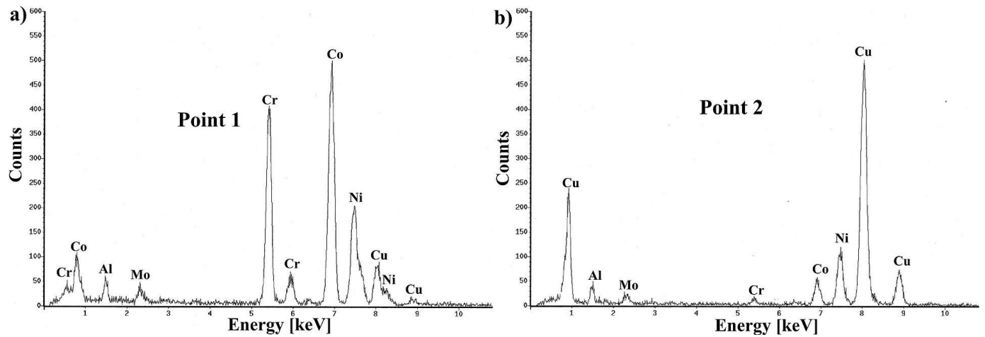
Fig. 8. EDS point analysis obtained from a) point 1 and b) point 2 of the TEM cross-section image of AlCoCrCuNi after oxidation at 1273 K in air for 24 h
