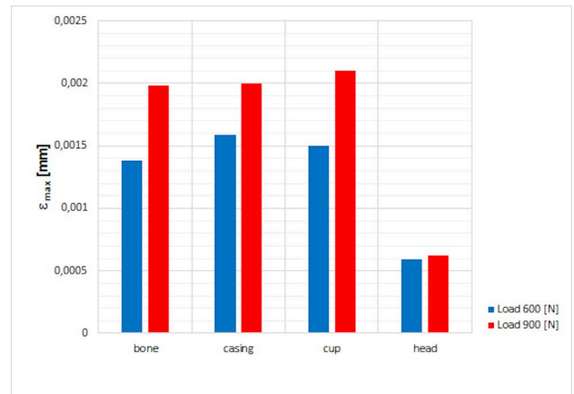
Fig. 8. Statements of the values of strain in the analysed system with the load 600 N and 900 N
