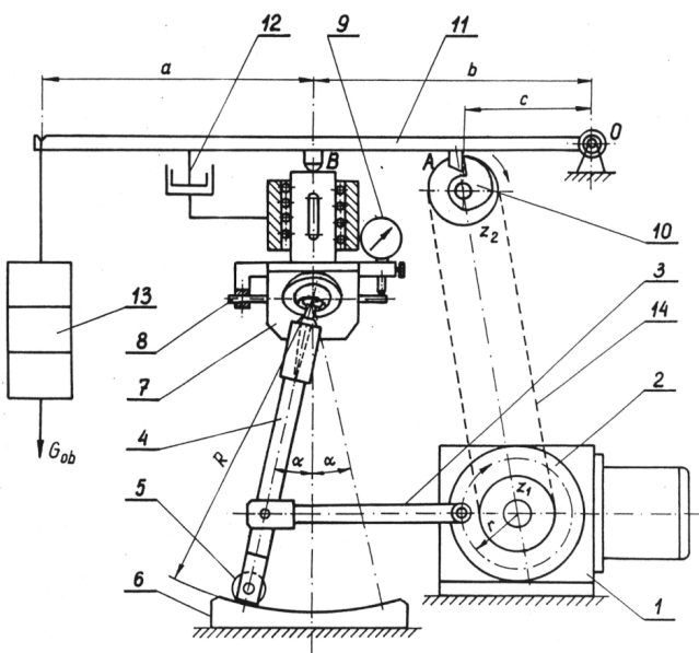
Fig. 9. Schematic diagram of the stand for testing durability of human hip joint endoprosthesis [15]
