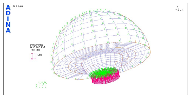
Fig. 3. Model of discreet elaborated solution
