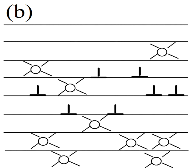
Fig. 7. (a) Sodium penetration induced dislocation array in area 3 for the carbon cathode (b) explaining the presence of the dislocation array
