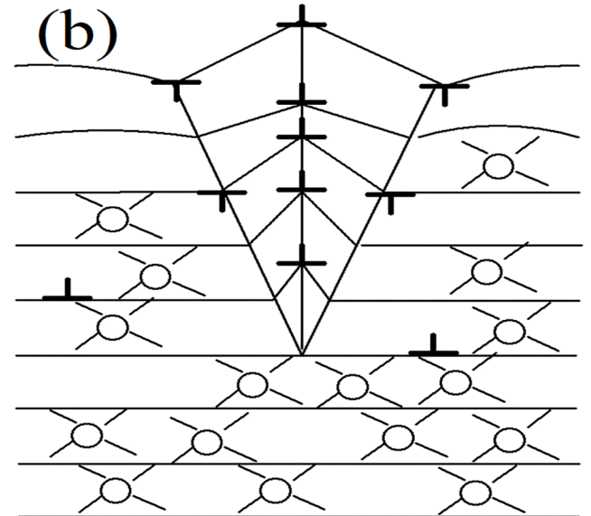
Fig. 9. (a) The 60° orientation relationship between kink bands induced by sodium penetration in area 1 for the carbon cathode (b) explaining the 60° orientation relationship between kink bands
