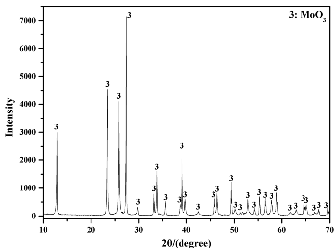
Fig. 1. XRD pattern of raw material MoO 3
