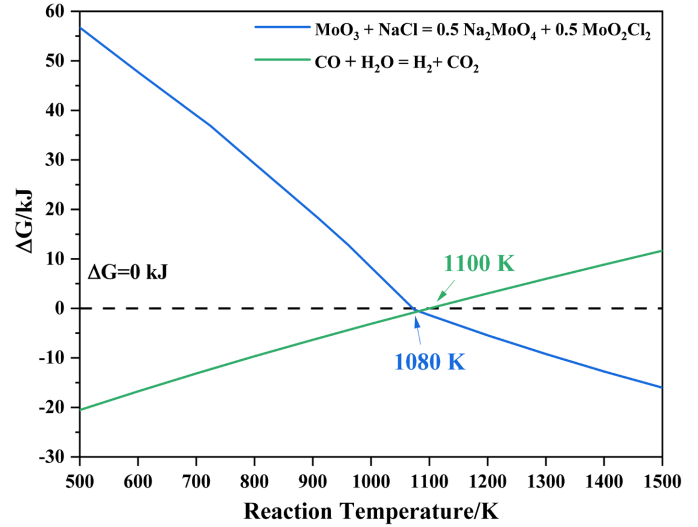
Fig. 8. The standard Gibbs free energy changes for Eqs. (4) and (9)
