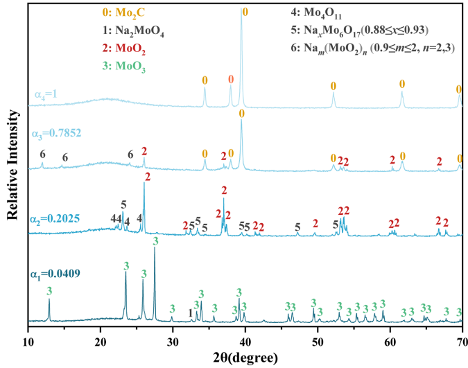
Fig. 7. XRD patterns of the reaction products obtained by reducing 2 wt.% NaCl-doped mixed \text{MoO}_3 with high-purity CO gas at different stages
