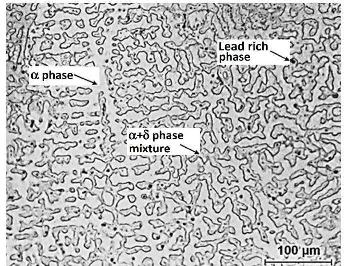
Fig. 3. Metallographic structure of SAE 660 leaded bronze
