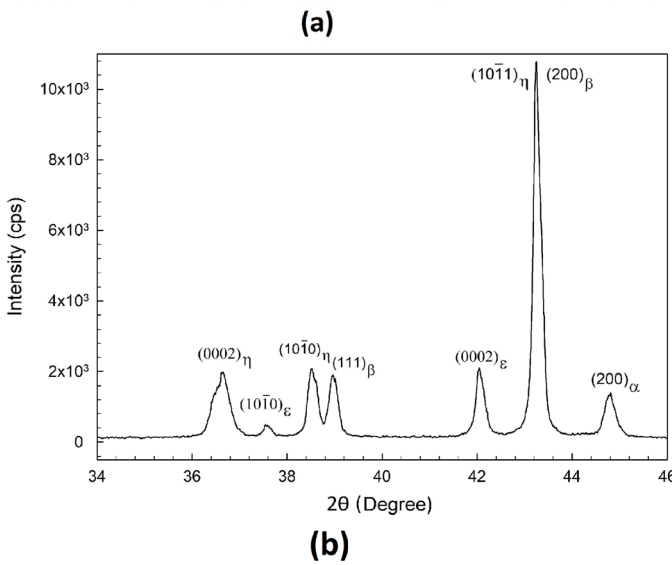
Fig. 2. (a) Metallographic structure and (b) X-ray diffraction pattern of Zn-30Al-3Cu alloy
