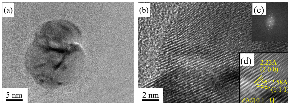
Fig. 9. TEM analysis of NbC precipitates. (a) Bright field, (b) HRTEM images of precipitates, (c) FFT diagram of the micrographs in (b), (d) FFT filtered images derived from the images (b)
