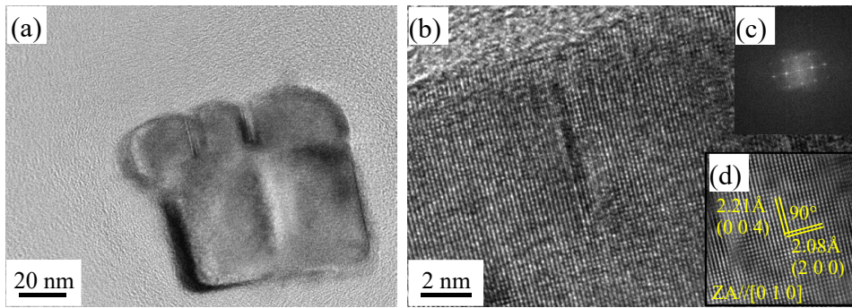
Fig. 8. TEM analysis of Ti_2N precipitates. (a) Bright field, (b) HRTEM images of precipitates, (c) FFT diagram of the micrographs in (b), (d) FFT filtered images derived from the images (b)
