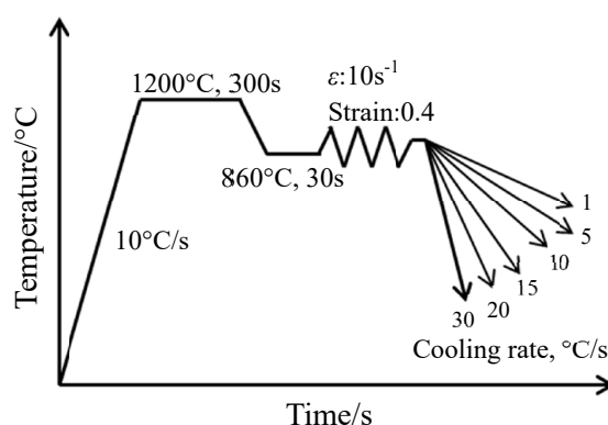
Fig. 1. Thermal simulation procedure of the X70 pipeline steel
