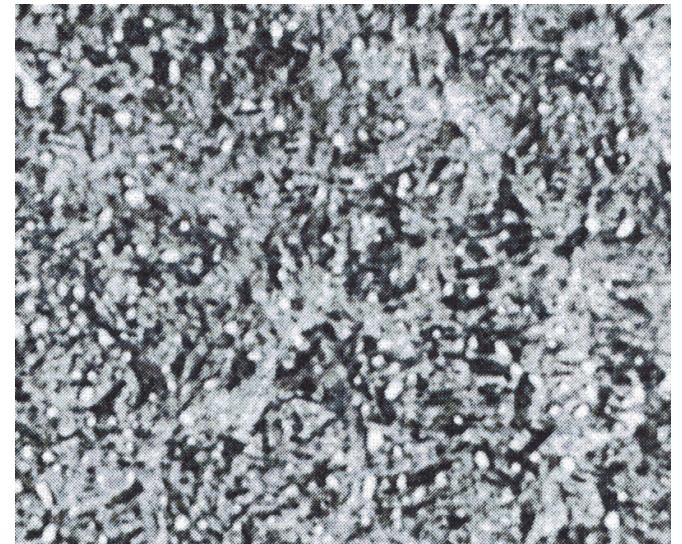
Fig. 10. Micro-structure of bearing race of Renault Kangoo wheel, magnification 100x, surface etched by nital
