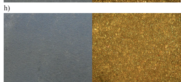
Fig. 2. Macro- and microscopic observation of the surface of the Al-Si coating without and after heat treatment
