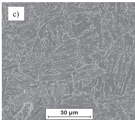
Fig. 1c. SEM – Tempered martensite with carbides precipitates along the borders of martensite lamellae and former austenite grains.
