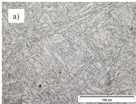
Fig. 1a. LM – P92 steel microstructure. Tempered martensite with visible non-metallic inclusions.
