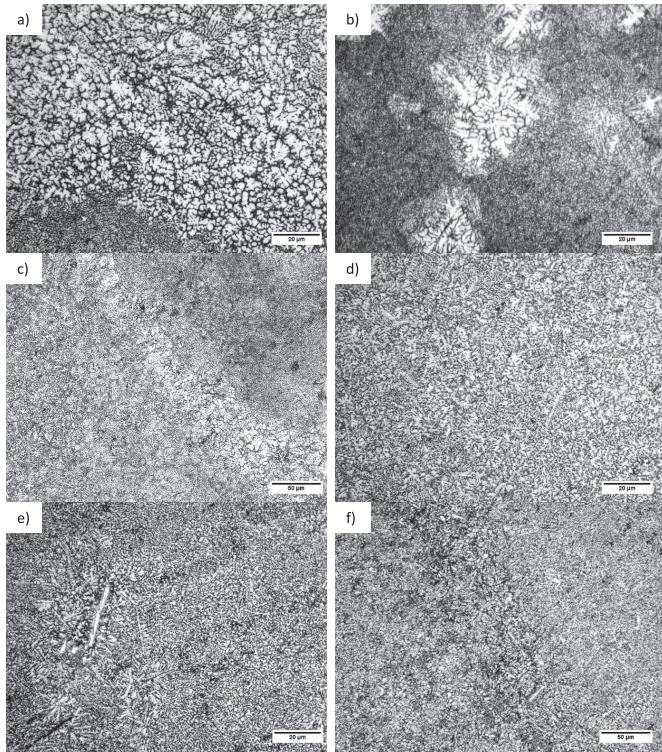
Fig. 2. Microstructures of titanium alloy Ti6Al4V a), b) and c) produced by injection method with suction under vacuum atmosphere d), e) and f) produced by injection method with suction in air atmosphere, respectively
