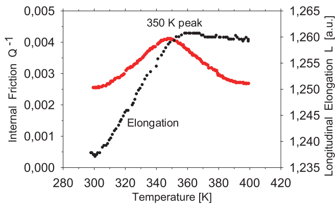
Fig. 4. Internal friction peak at 350 K in a Fe-C alloy after 4 % cold-work at 77 K, accompanied by longitudinal elongation of the sample measured by the laser triangulation technique (the resonant frequency is 1.4 Hz)
