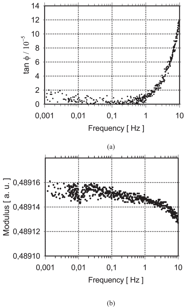
Fig. 1. The performance of the high-resolution mechanical spectrometer, HRMS. Variation of the \tan \varphi (a) and modulus (b) with frequency for the optimized number of oscillations, N_{osc} . The frequency sweep was measured in the range from 10 to 10^{-3} Hz. The signal-to-noise ratio S/N = 70 dB
