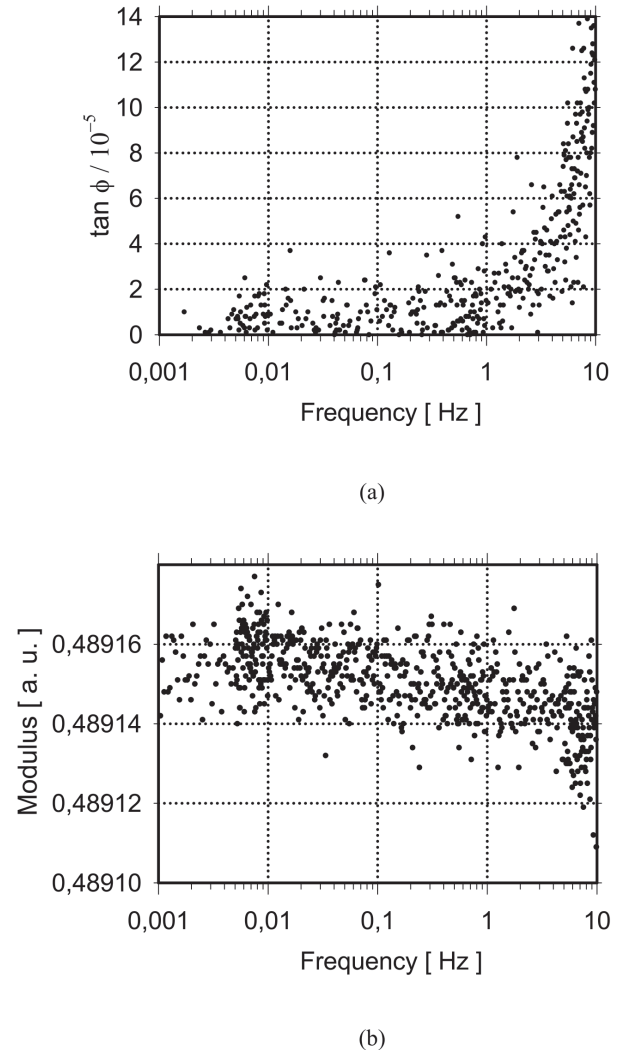
Fig. 2. The performance of the high-resolution mechanical spectrometer, HRMS. Variation of the \tan \varphi (a) and modulus (b) with frequency for a small number of oscillations, N_{osc} = 3 . The frequency sweep was measured in the range from 10 to 10^{-3} Hz. The signal-to-noise ratio S/N = 70 dB
