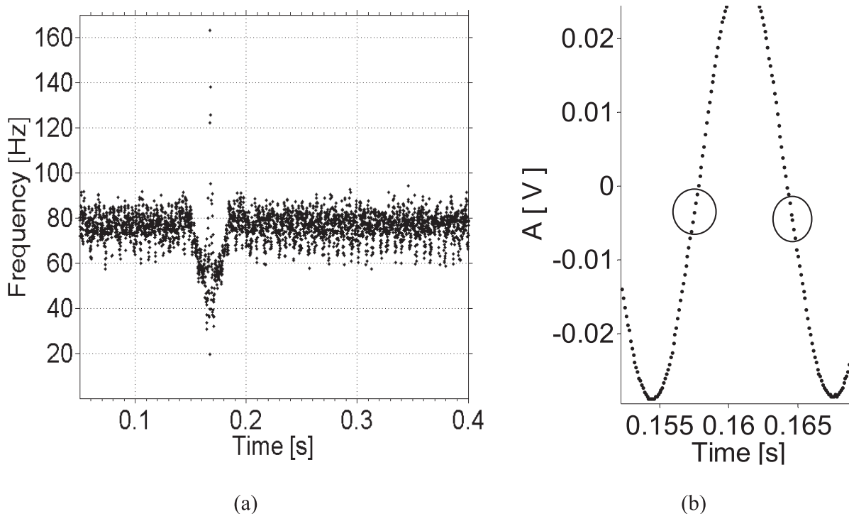
Fig. 3. The signal quality test of free decaying oscillations: \delta = 1.51 \times 10^{-2} , the resonant frequency f_0 \approx 76.39 Hz, the sampling frequency f_s = 10 kHz. (a) The time-frequency analysis yields a spike, which precisely localizes irregular sampling time-interval recorded by the ILD Micro-Epsilon instrument. (b) A zoom on the analyzed free decaying oscillations indicates an irregular sampling time-interval
