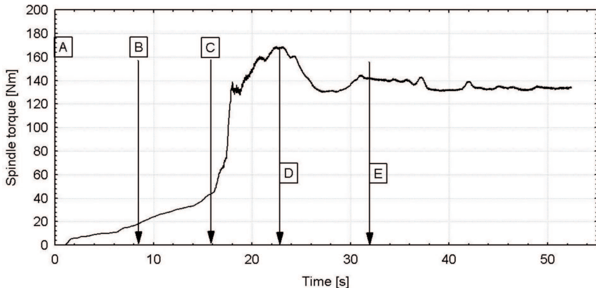
Fig. 7. Spindle torque signal recorded during FSP ( \omega=450 rpm, v=224 mm/min)
