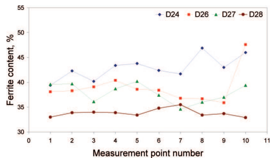
Fig. 12. Influence of heat input on ferrite content on weld root in test welded joints: D24, D26, D27, D28 (Table. 2) lean duplex S32101 plates of thickness 12 mm
