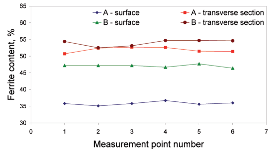
Fig. 8. Differences in ferrite measurements results on ground surface and in samples cross section area cut out of S32101 steel plates from different heat melts
