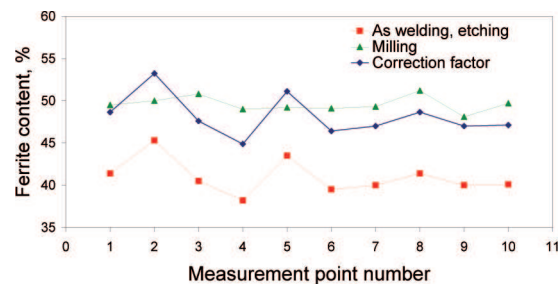
Fig. 13. Influence of root weld shape of S32101 steel and correction factor on measurement quantity of ferrite content
