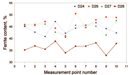
Fig. 11. Influence of heat input on ferrite content on weld face in test welded joints: D24, D26, D27, D28 (Table. 2) lean duplex S32101 plates of thickness 12 mm
