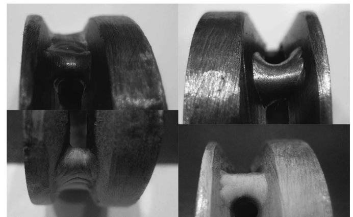
Fig. 13. Elimination of cracks by applying pre-heating to temperature of 150^{\circ}\text{C}
