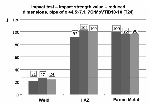
Fig. 5. Impact strength of weld metal in butt welded joints of T24 steel in tubes of \phi 44.5 \times 7.1
