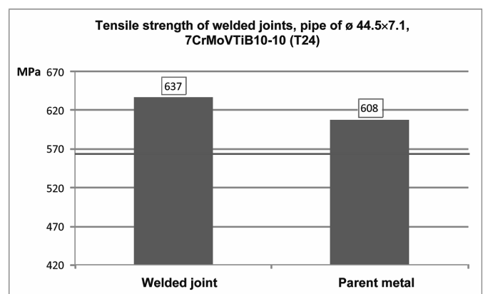
Fig. 4. Results of tensile test of butt welded joints of tubes of \phi 44,5 \times 7,1
