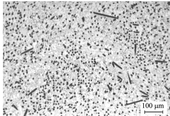
Fig. 1. Arrangement of chopped carbon fibres in composite containing 5% vol.reinforcing phase
