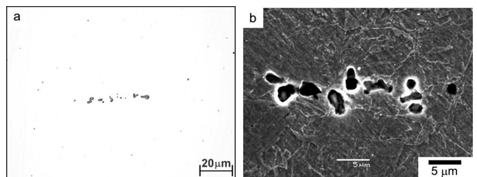
Fig. 4. Micrographs of non-metallic inclusions in W1 steel: a) optical microscopy, b) SEM
