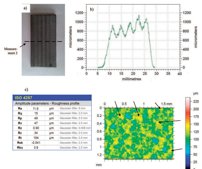
Fig. 6. Coating for trial 6: view of deposited coating (a), surface topography for measurement 2 (b), surface roughness from confocal microscope (c)
