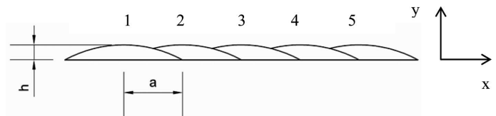
Fig. 3. Distribution scheme of coating with thickness h less than 1 mm obtained when spacing of spraying gun passes was a = 3.7 mm
