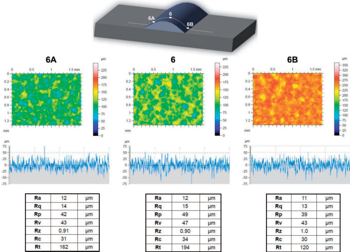
Fig. 7. Roughness measurements with confocal microscope for three bead points
