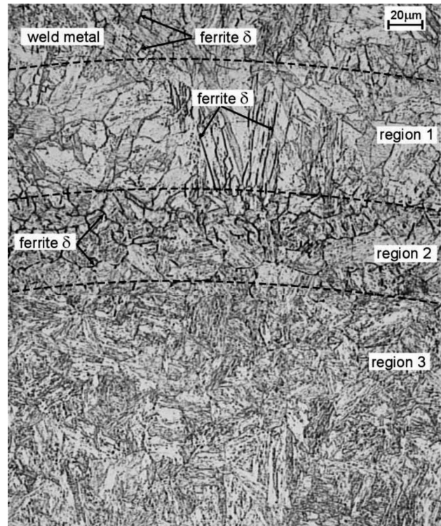
Fig. 4. Microstructure near the fusion line and the high-temperature regions of the HAZ from the place marked "A" in Fig. 3
