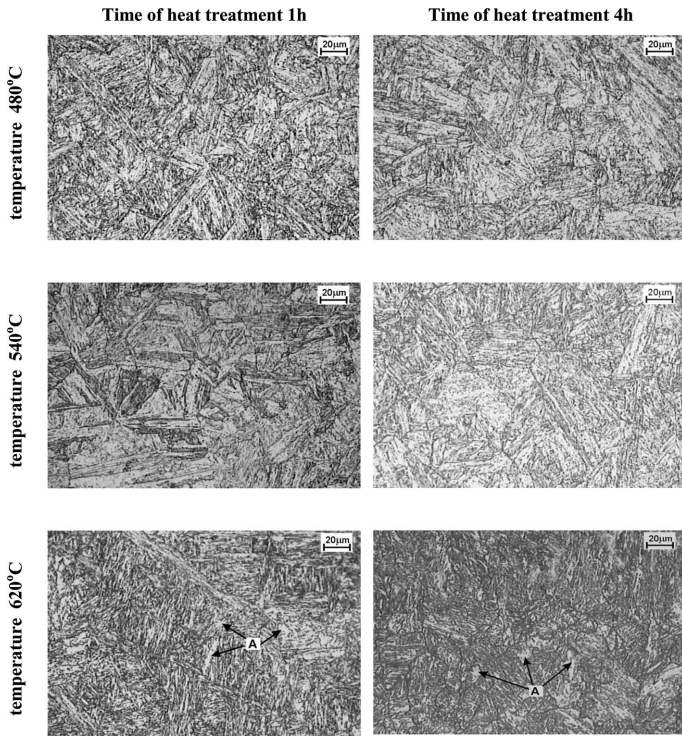
Fig. 6. Base metal microstructure after heat treatment. The bright regions visible between the plater of austenite (marked by arrows and capital letter “A”)
