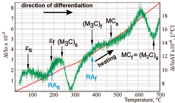
Fig. 2. Dilatogram and its first derivative for HS18-0-1 steel heated from as-quenched state at 0.05°C/s, Adamel-Lhomargy DT1000 dilatometer [2]
