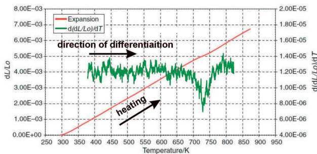
Fig. 4. Expansion curve and its derivative of an as-quenched 17-4 PH steel sample, 2 K min -1 heating rate, Netzsch 402 ES dilatometer [4]
