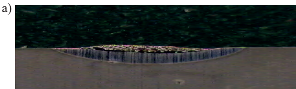
Fig. 5. The cross - section of laser surface alloyed X40CrMoV5-1 steel after laser alloying with a) WC powder and b) VC powder at laser beam power of 2.3 kW
