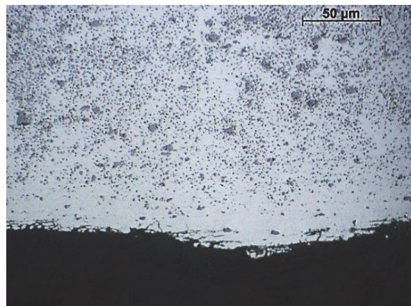
Fig. 7. Structure of the AlSiCu3 PM material anodised surface layer with 5% \text{Al}_2\text{O}_3 powder addition
