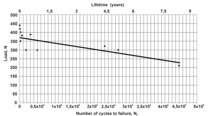
Fig. 8 The load-cycle diagram the fatigue limit of the implantological system with the zirconia abutment
