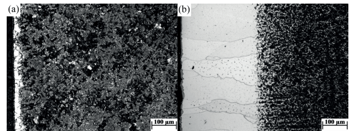
Fig. 5. Surface decarburization after heating at 760 °C: (a) 5 min, water quenching; (b) 4 h, air cooling
