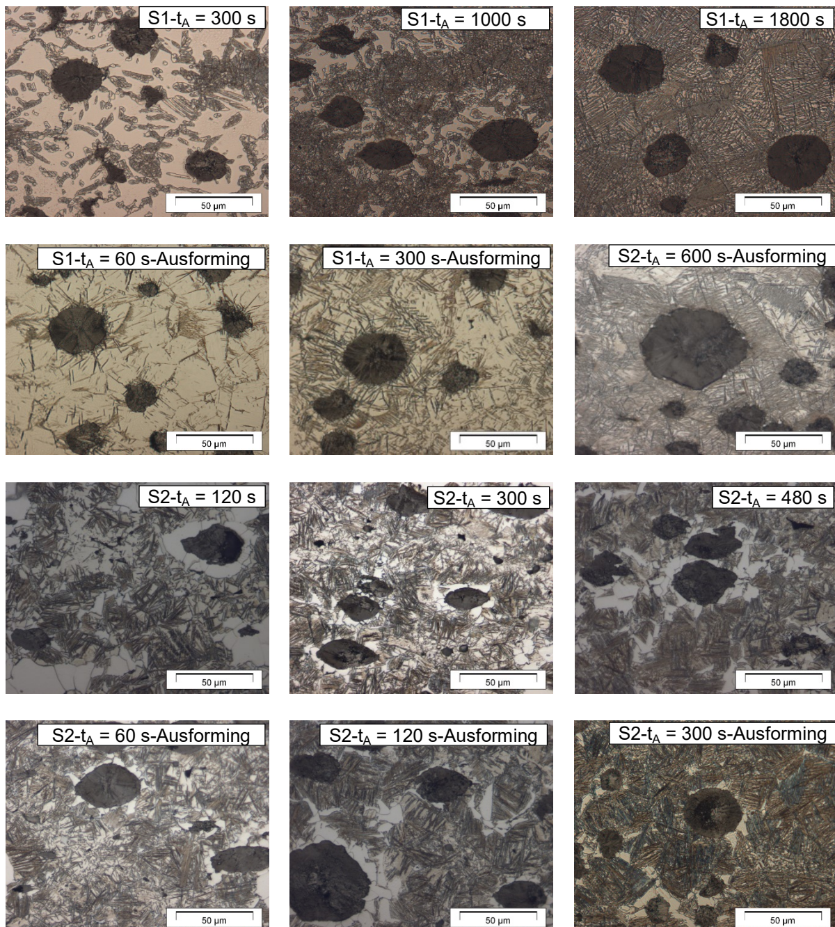
Fig. 4. Micrographs showing acceleration of kinetics of ausferrite formation due to the ausforming process and introduction of ferrite to the matrix of DI. t_A : holding time after quenching to T_A
