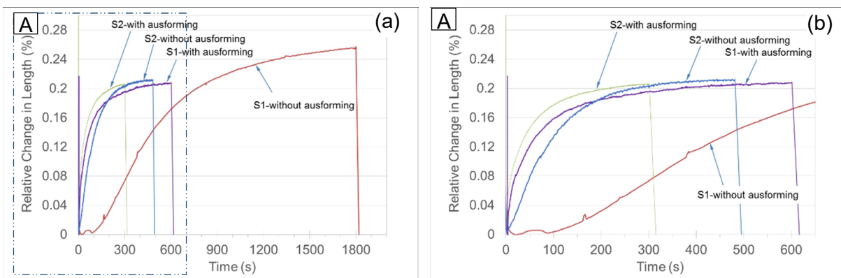
Fig. 3. Kinetics of ausferrite formation for the prescribed processing techniques. In (b) details of section A
