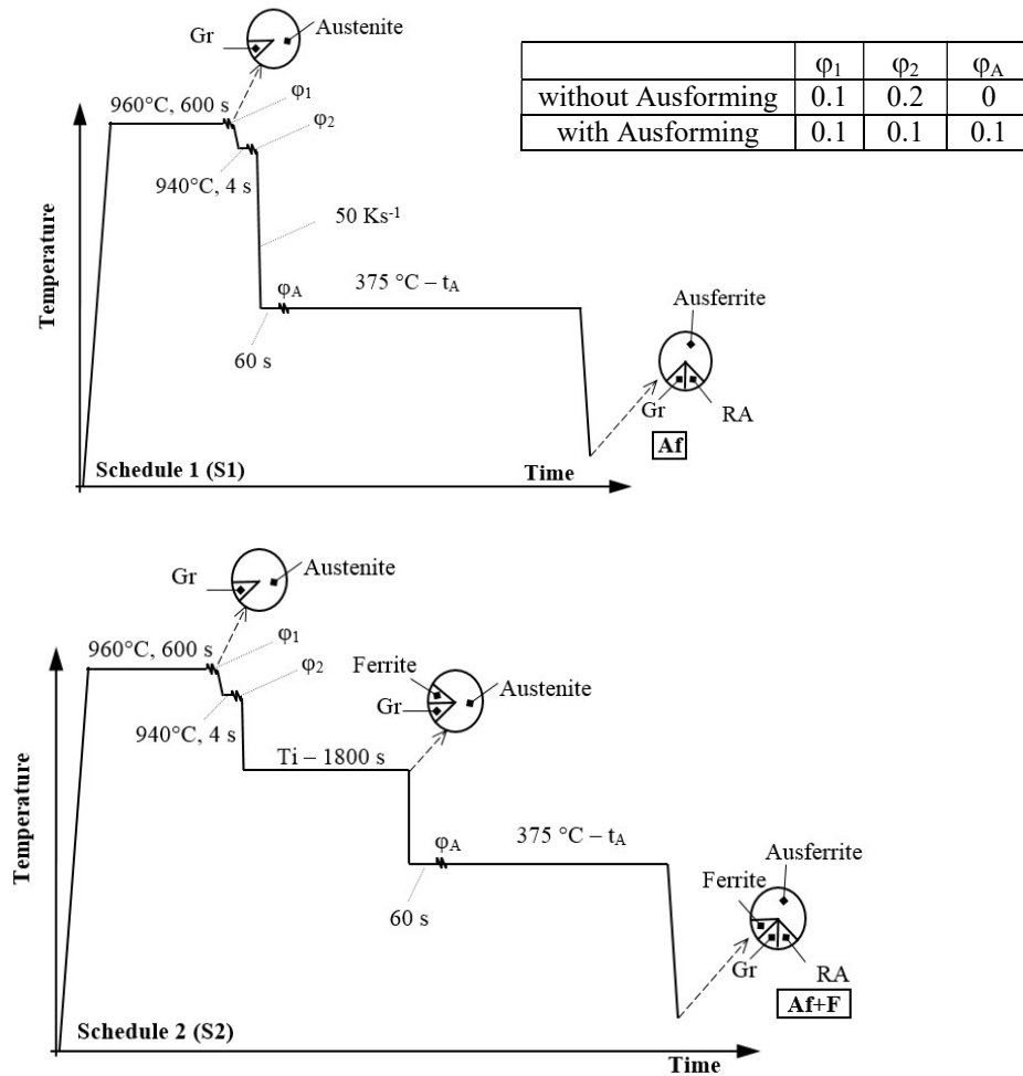
Fig. 2. Thermo-mechanical schedules applied to the four ductile irons, Gr: graphite, RA: retained austenite and T_A : austempering temperature
