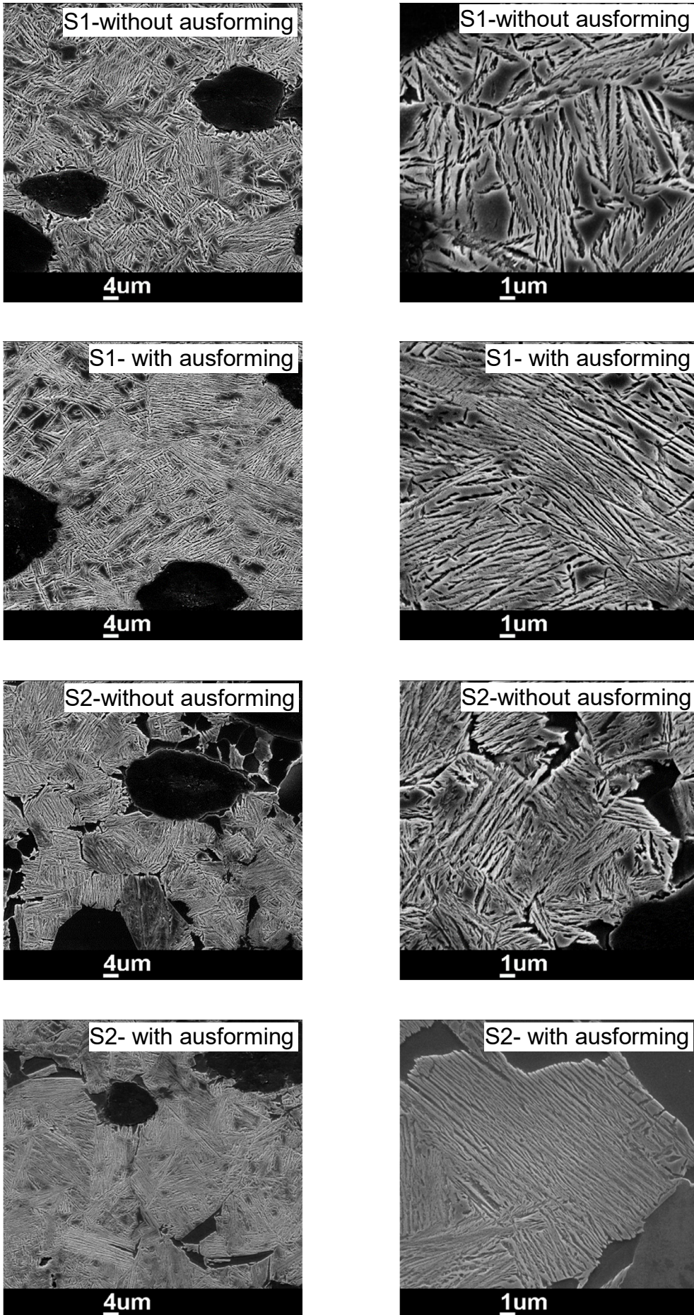
Fig. 5. SEM structures observed after quenching of the prescribed processing conditions
