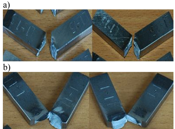
Fig. 8. A view of broken impact samples of the test joint A (a) and test joint B (b), Table 4
