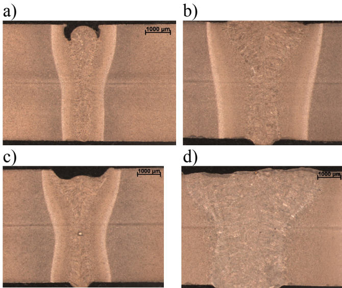
Fig. 4. Macrostructure on cross sections of the bead-on-plate welds produced on 5.0 mm thick plates of STRENX 1100 MC steel by the Disk laser TRUMPF TruDisk 3302, Table 2; a) bead No. 1 (99 J/mm), b) bead No. 2 (198 J/mm), c) bead No. 3 (132 J/mm), d) bead No. 4 (396 J/mm)
