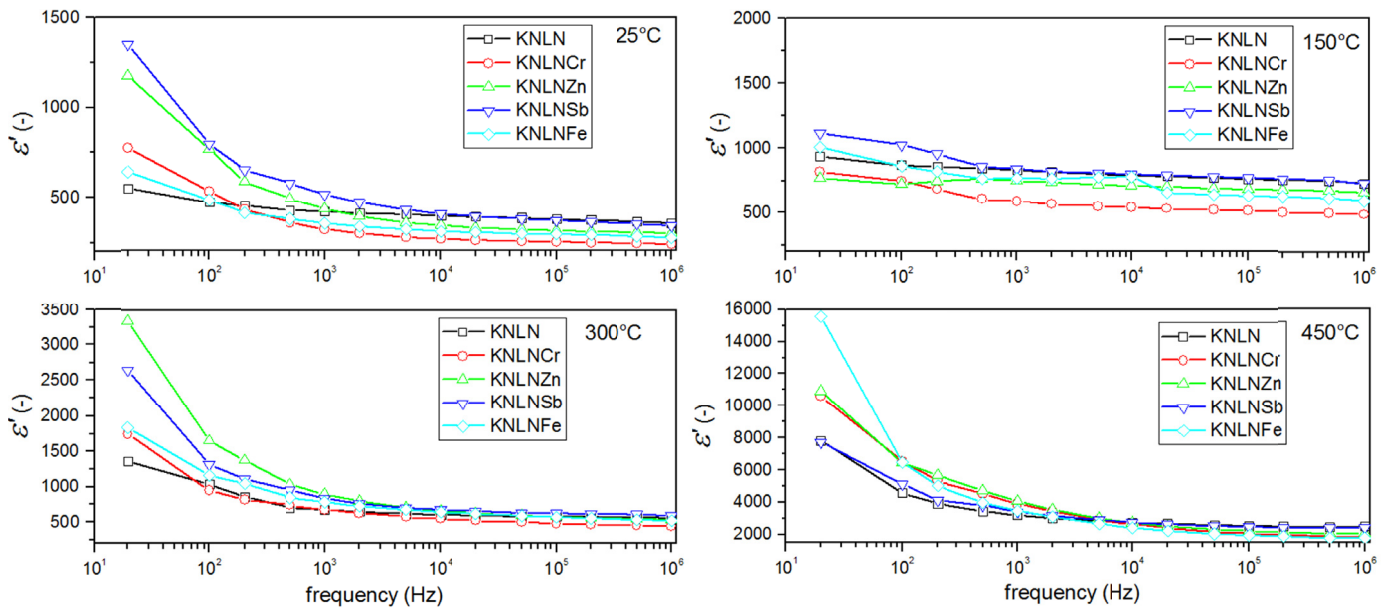
Fig. 7. Frequency dependence of dielectric permittivity for KNLN-type samples at different temperatures
