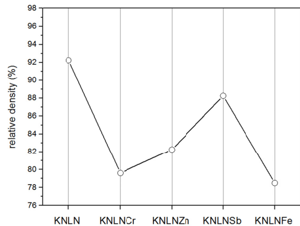
Fig. 1. The relative density RD of the KNLN-type ceramics
