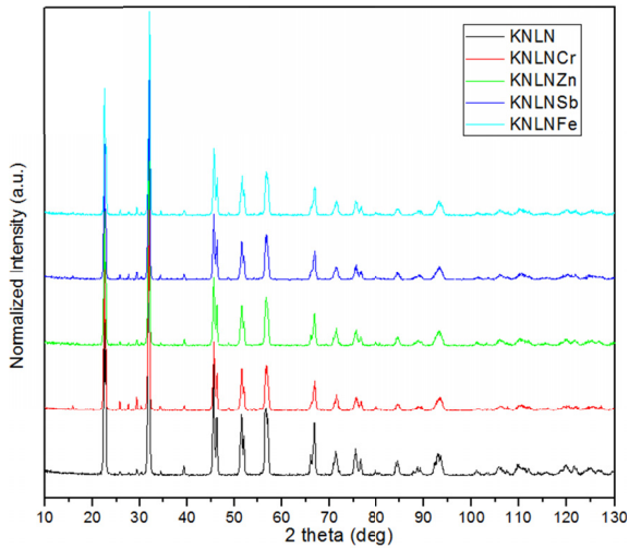
Fig. 2. The XRD patterns of the KNLN-type ceramics
