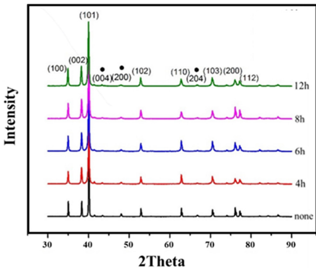
Fig. 1. XRD peak analysis of cryomilled powder depending on milling time
