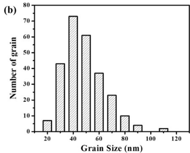
Fig. 3. (a) TEM micrograph and (b) grain size histogram measure from TEM micrograph of 8 hour cryomilled powder
