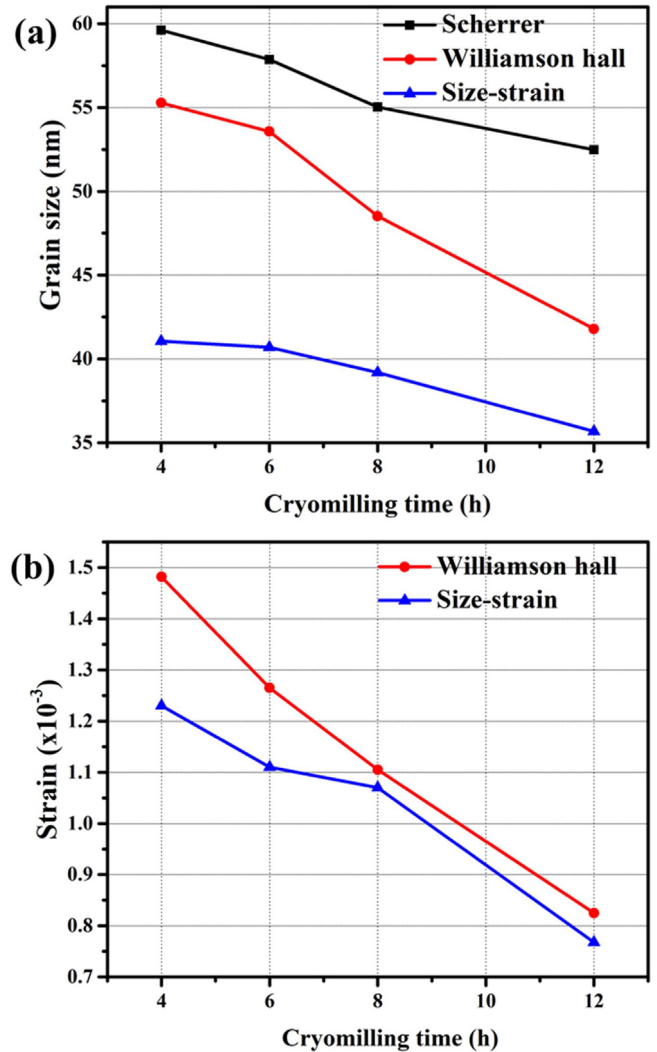
Fig. 2. Comparison of (a) grain size and (b) lattice strain data obtained from three different calculation methods
