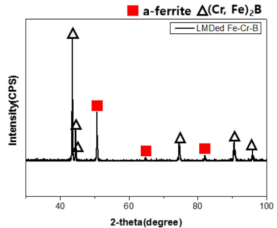
Fig. 2. X-ray diffraction analysis results of Fe-Cr-B alloy fabricated with laser metal deposition
