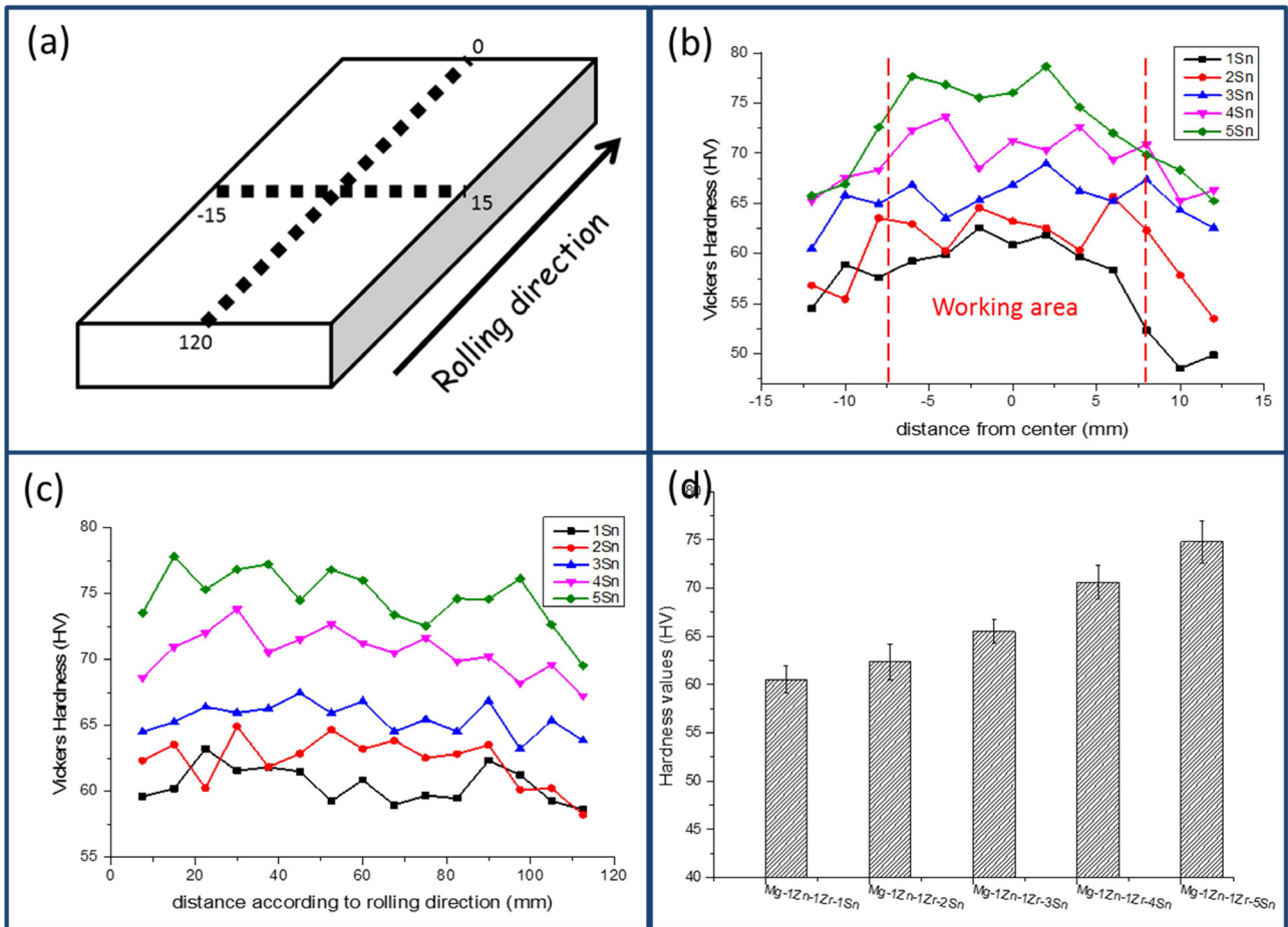
Fig. 5. (a) Schematic representation of the Vickers hardness measurement according to the rolling direction, and the Vickers hardness of the alloys according to (b) cross-sectional area, (c) along the rolling direction, and (d) average Vickers hardness of the alloys processed by PTR
