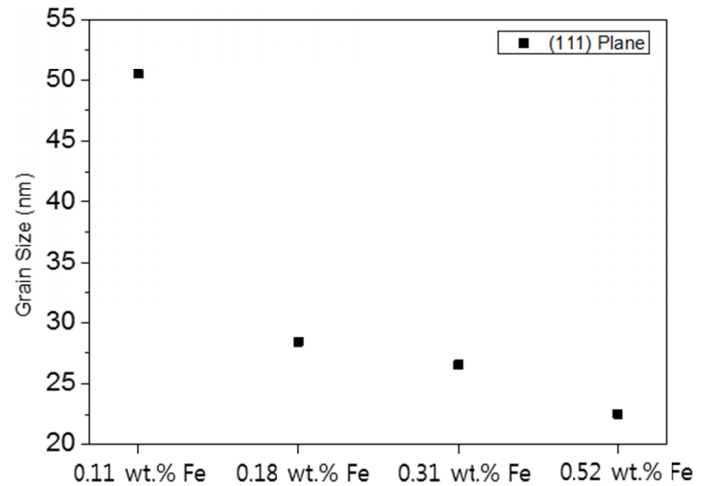
Fig. 6. Grain size of electroplated Au-Fe alloy layers with respect to the Fe content
