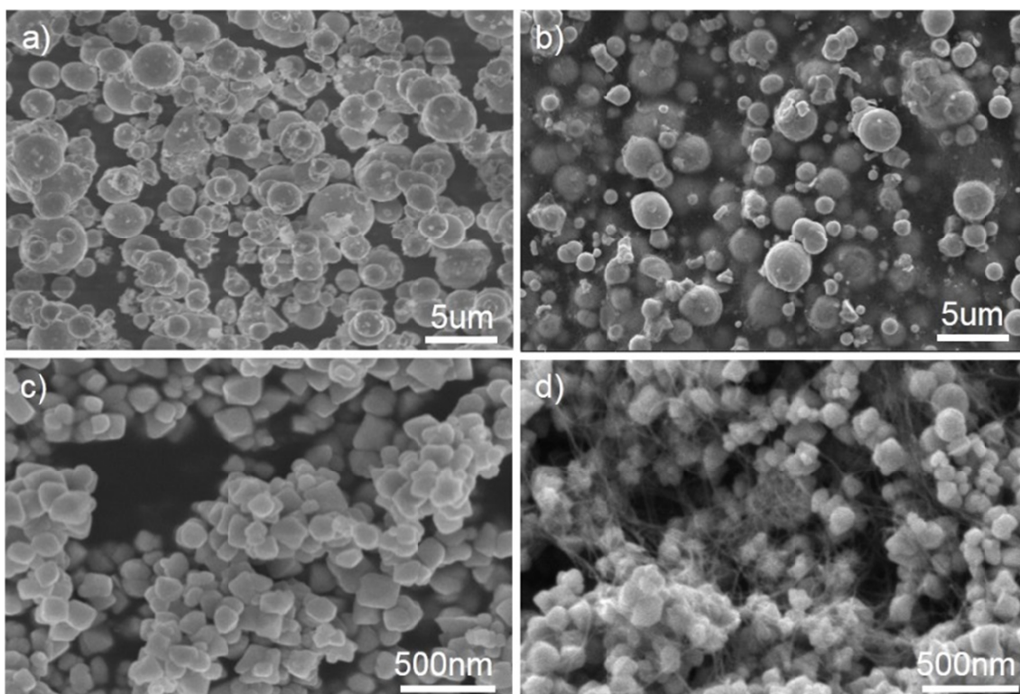
Fig. 1. SEM image of a) CI, b) CI/CNT, c) \text{Fe}_3\text{O}_4 , and d) \text{Fe}_3\text{O}_4 /CNT, respectively
