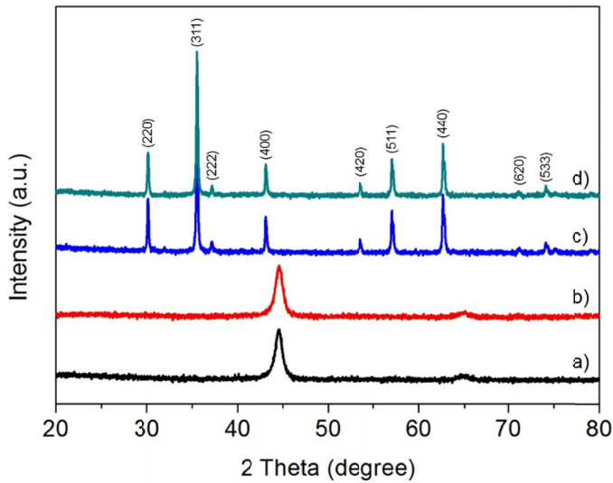
Fig. 2. XRD peaks of a) CI, b) CI/CNT, c) Fe 3 O 4 , and d) Fe 3 O 4 /CNT, respectively
