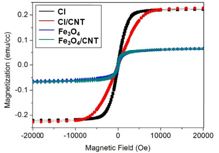
Fig. 3. SQUID measurements of CI, CI/CNT, Fe 3 O 4 , and Fe 3 O 4 /CNT
