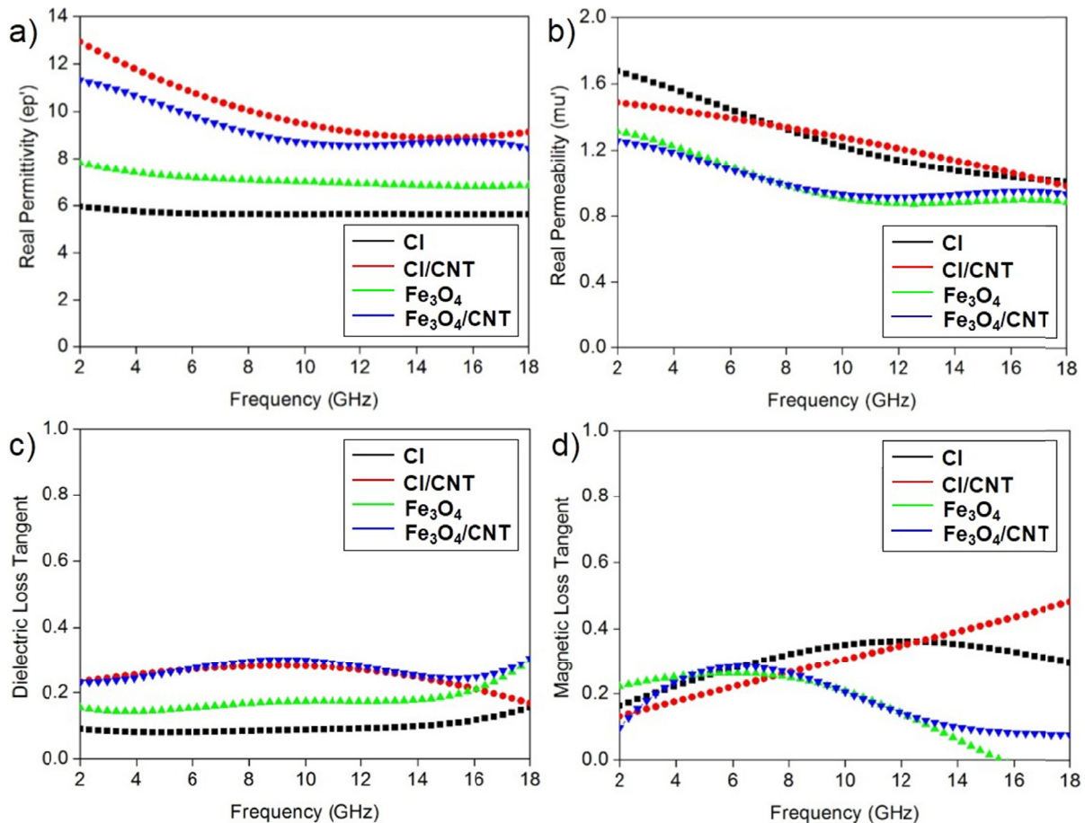
Fig. 4. a) Real permittivity of CI, CI/CNT, Fe 3 O 4 , and Fe 3 O 4 /CNT, b) Real permeability of CI, CI/CNT, Fe 3 O 4 , and Fe 3 O 4 /CNT, c) Dielectric Loss Tangent of CI, CI/CNT, Fe 3 O 4 , and Fe 3 O 4 /CNT, and d) Magnetic Loss Tangent of CI, CI/CNT, Fe 3 O 4 , and Fe 3 O 4 /CNT
