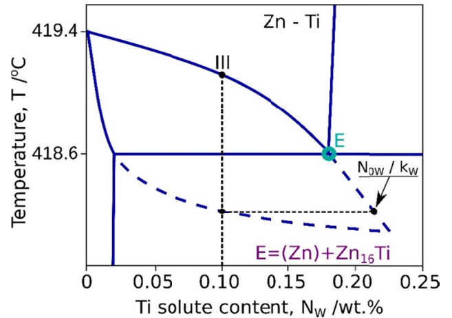
Fig. 3. The nominal Ti – solute concentration (“III”), N_{0W} \equiv III = 0.1 , [wt.%], and the position of the III \rightarrow E \rightarrow N_{0W}/k_W – path for the equilibrium solidification (partially speculative)
