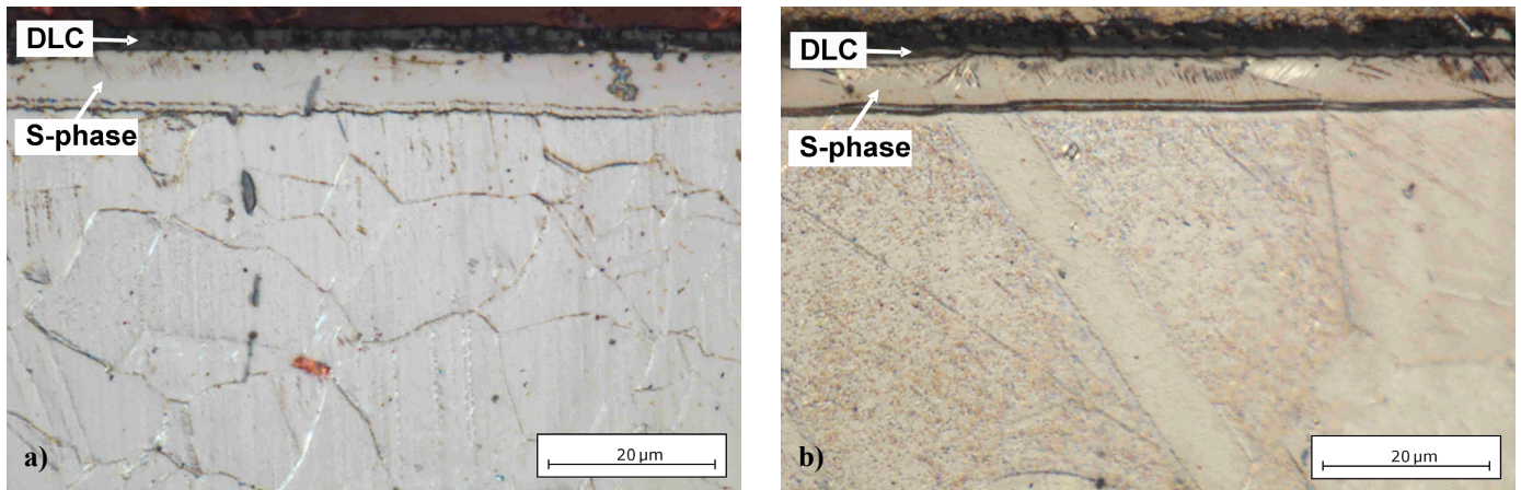
Fig. 1. Microstructure of DLC coatings produced in (a) DC and (b) pulsed glow discharge conditions on nitrided 316L steel
