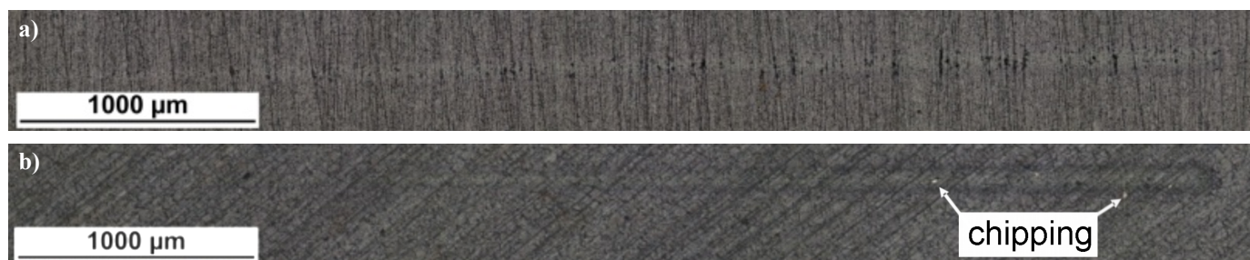
Fig. 3. Scratch images of DLC coatings produced in (a) DC and (b) pulsed glow discharge conditions on nitrided 316L steel
