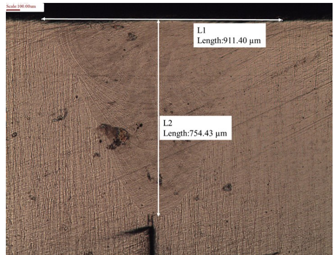
Fig. 6. Resolidified zone for case of continuous electron beam welding in cross-sectional view
