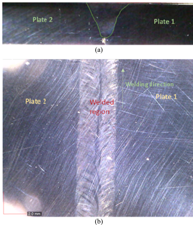
Fig. 5. Experimental image of continuous electron beam butt welding (a) cross-sectional view (b) top view
