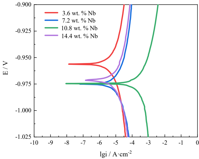
Fig. 5. Polarization curve of self-shielded metal-cored arc welding overlays with different niobium additions in 3.5 wt.% NaCl solution + 0.01 mol/L HCl solution
