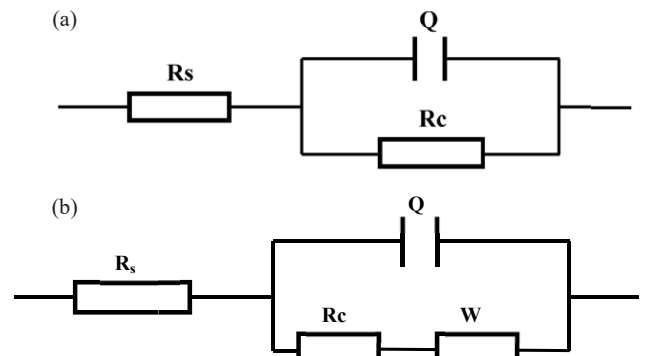
Fig. 8. Equivalent circuit model for the impedance spectra measured in 3.5 wt.% NaCl solution + 0.01 mol/L HCl solution (a) for 3.6 wt.% Nb, 7.2 wt.% Nb and 14.4 wt.% Nb, (b) for 10.8 wt.% Nb
