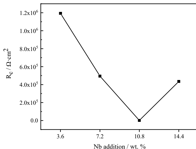
Fig. 9. Change trend of R_c values for welding overlays with different niobium additions
