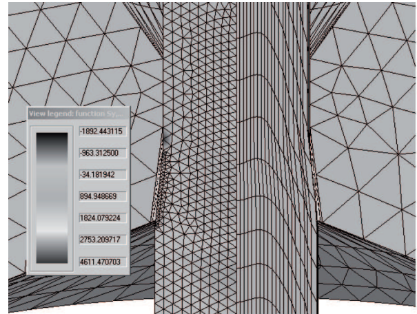
Fig. 2. The example of the distribution of longitudinal stresses \sigma_y in the final wire \phi 1.6 mm drawn according to variant A (classical dies)
