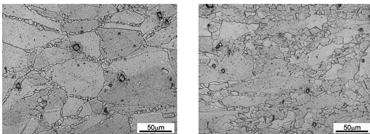
Fig. 9. Microstructure of a sample from Inconel 718 – after die forging at 1000°C, in two different sample areas (a) 1 and (b) 5
