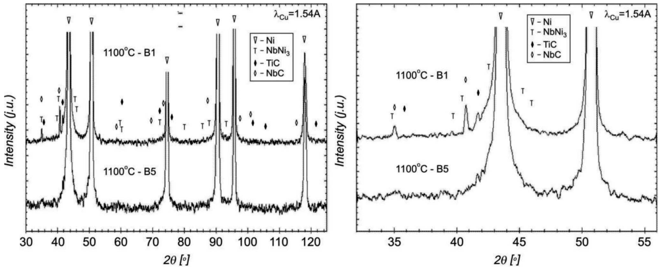
Fig. 5. Diffractogram of a sample from Inconel 718 alloy, after forging at the temperature of 1100°C, in the areas indicated 1 and 5 (2θ range 30-125°, and 30-55° with variable intensity scale to highlight the diffraction lines of phases with lower participation)
