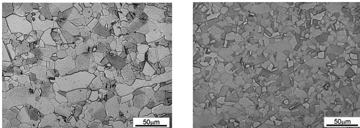
Fig. 8. Microstructure of a sample from Inconel 718 – after die forging at 1100°C, in two different sample areas (a) 1 and (b) 5
