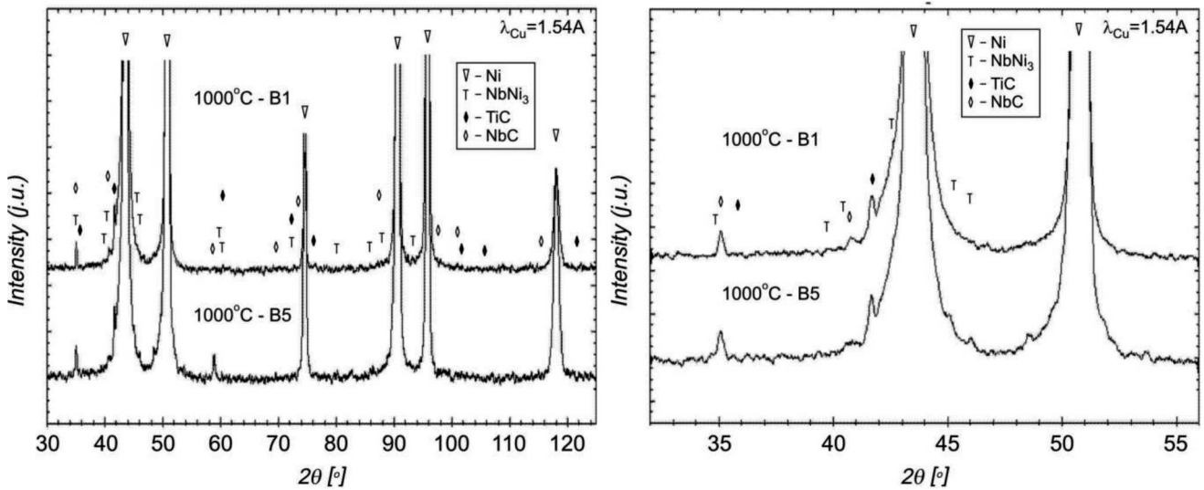
Fig. 6. Diffractogram of a sample from Inconel 718 alloy, after forging at temperature of 1000°C, in the areas indicated 1 and 5 (2θ range 30-125°, and 30-55° with variable intensity scale to highlight the diffraction lines of phases with lower participation)
