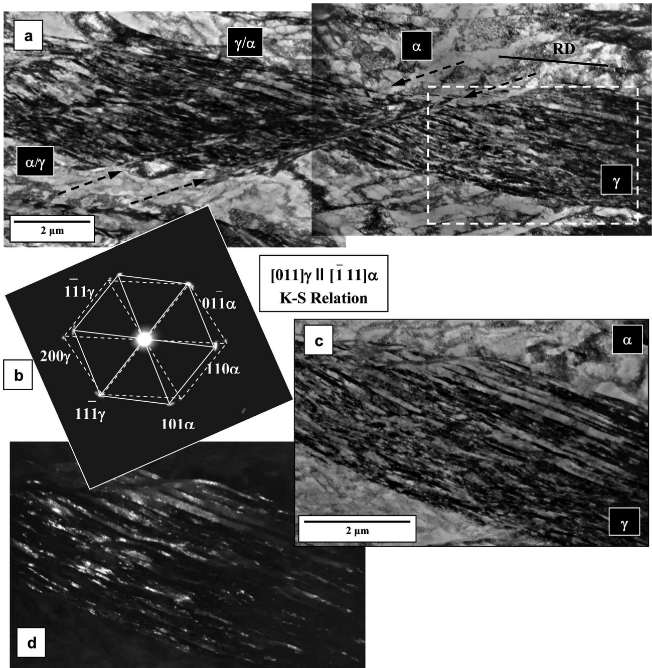
Fig. 10. Strongly refined lamellar-like microstructure within the austenite band after 80% of rolling reduction ( a , c ) and dark field analysis ( b , d ) indicating at ( \gamma \rightarrow \alpha ) transformation
